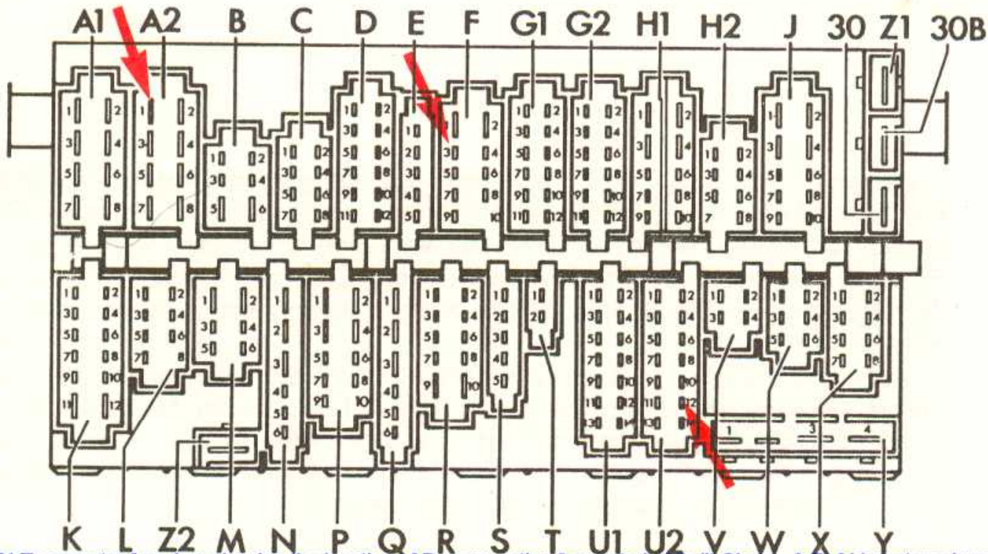
T4 Transporter fuse box showing the location of D+ connection for control of Split Charge & Refrigerator relays use A2 Pin1 if possible.
